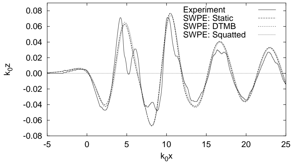
Figure 13: As above but with Froude number 0.4136.
